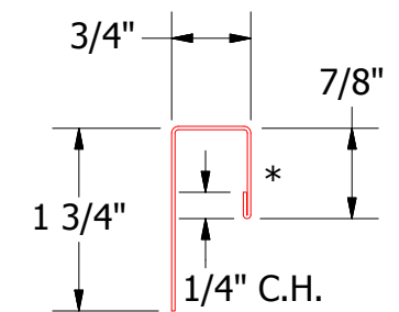
BGA034 - J Channel
