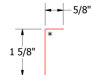
BGA680 - Angle Trim
