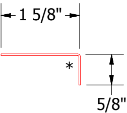
BGA680 - Angle Trim
