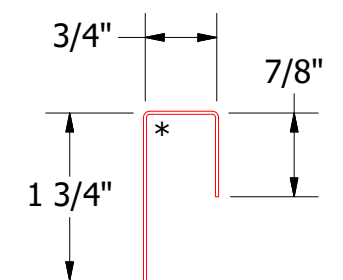
BGA270 - J Closure
