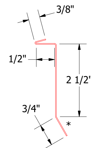
HLA980-Counterflashing
