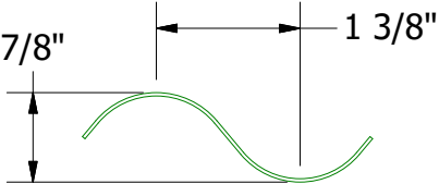
MCA682 Corra-Lok Profiled Support Z
