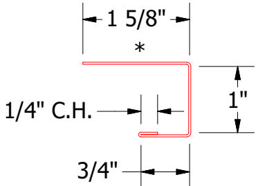
MCA118 - J Channel
