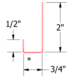
Perforated J Channel
