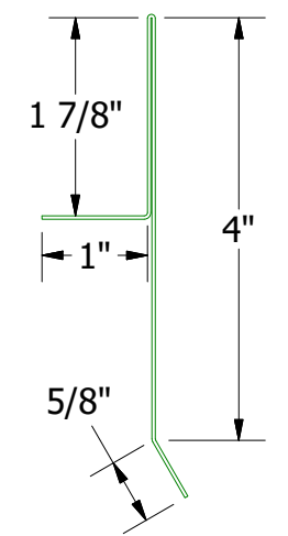
Gable Starter Cleat
