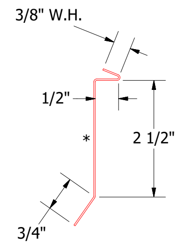
Counterflashing
