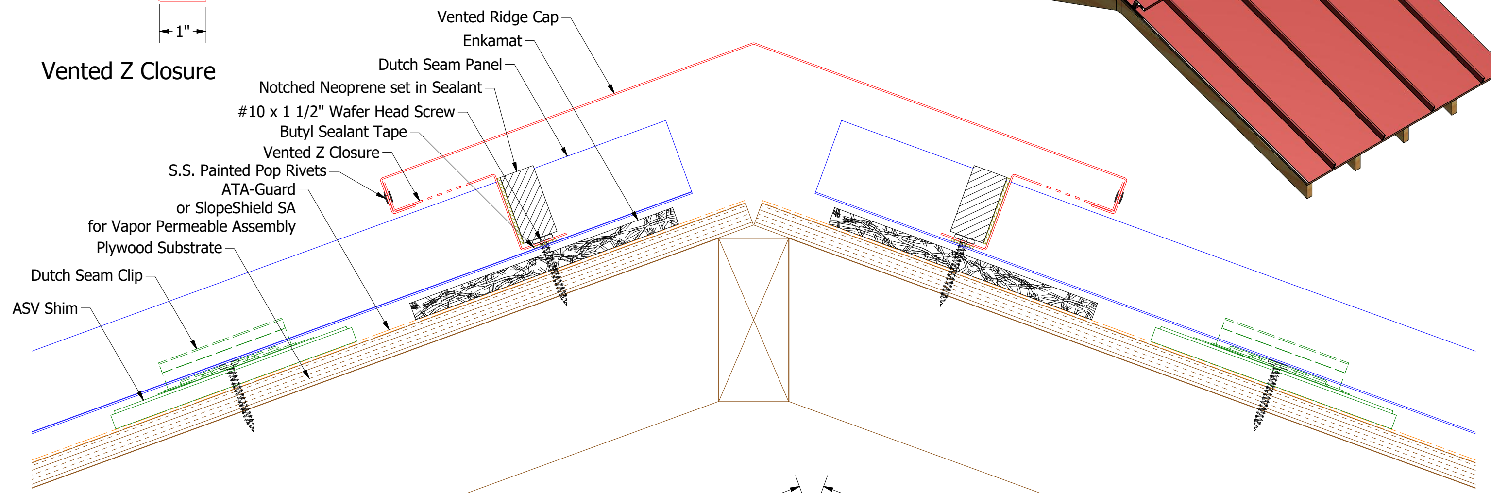
Factory Vented Pre Notched Z Closure 11" Panel - Factory Vented Pre Notched Z Closure will cover 5 Panels. 15" Panel - Factory Vented Pre Notched Z Closure will cover 4 Panels. 19 1/4" Panel - Factory Vented Pre Notched Z Closure will cover 3 Panels.
