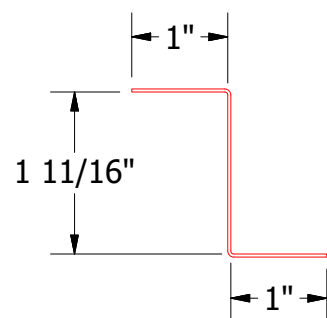
Z Closure
