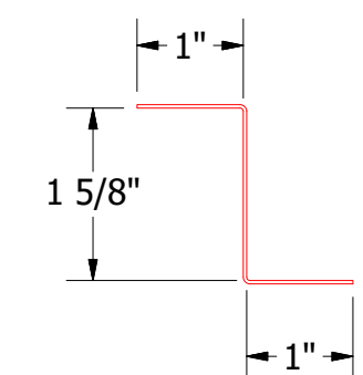
Z Closure
