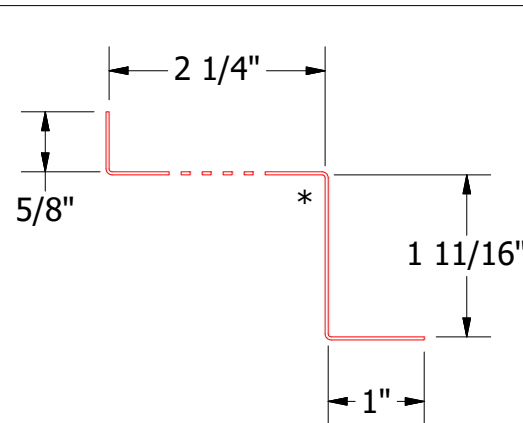
Vented Z Closure
