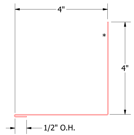
Sidewall Trim
