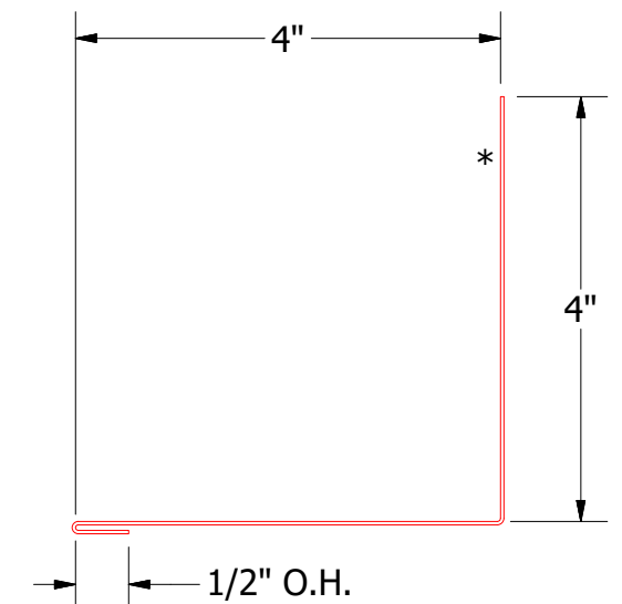
Sidewall Trim
