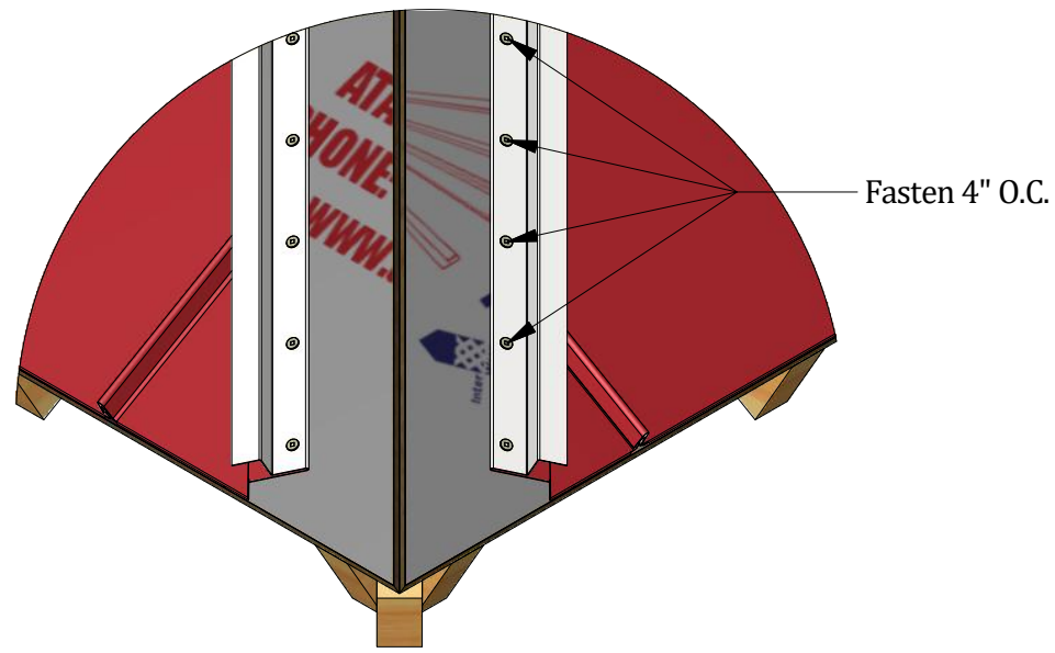
DETAIL - A
