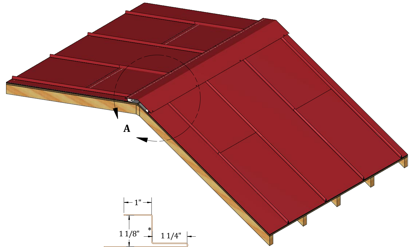
Pocket Z-Closure
