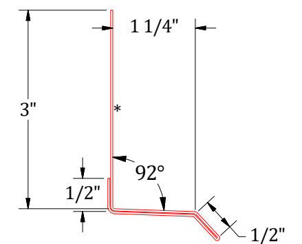
(300PD) Base Trim w/ Return
