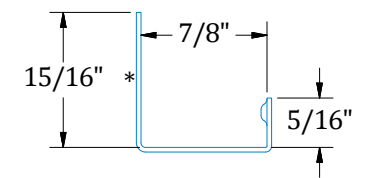
(HSA999) Custom HSS Snap R-Cover
