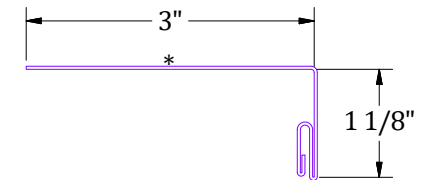
(130.1PB) Snap Base w/ I.S. Snap
