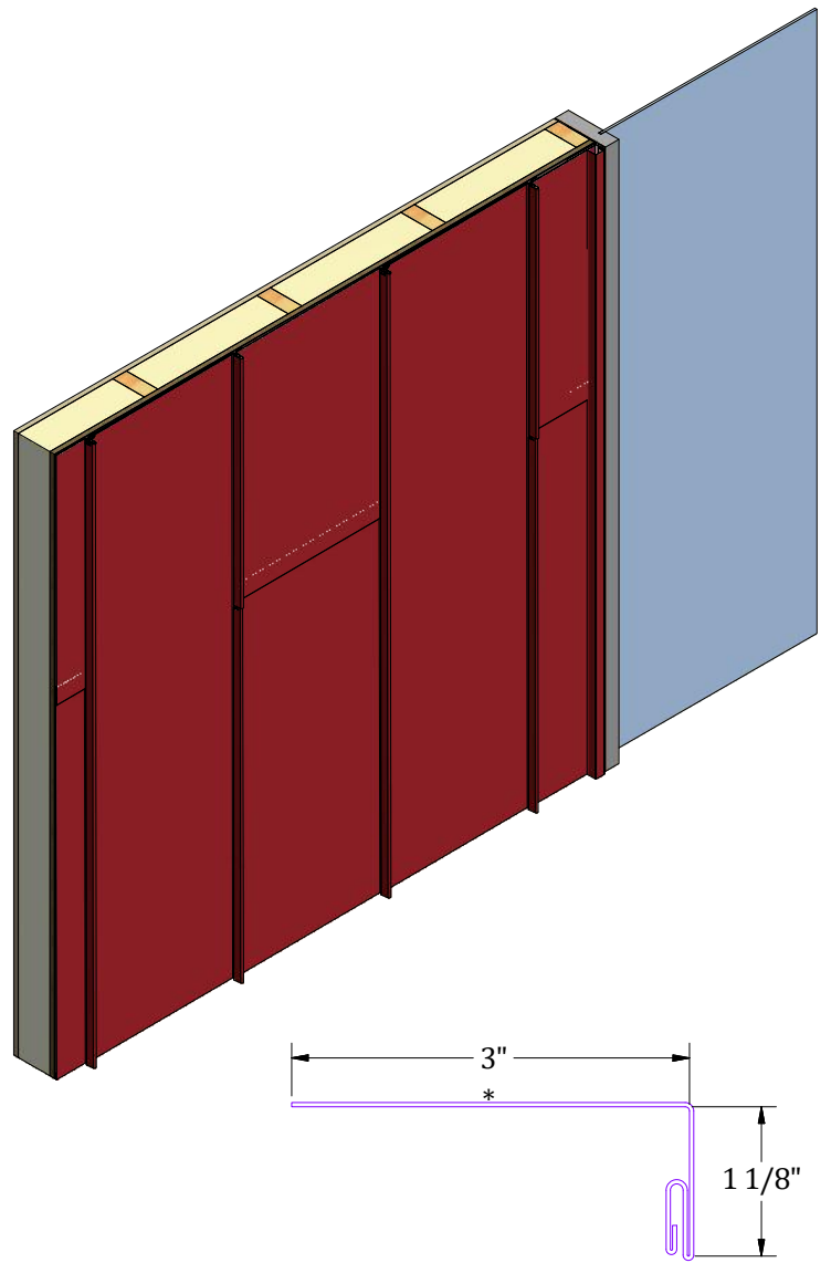
(130.1PB) Snap Base w/ I.S. Snap
