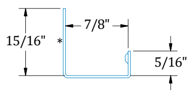
(HSA999) Custom HSS Snap R-Cover
