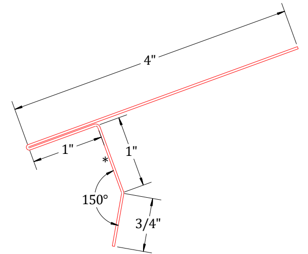
(602A) Flat Eave Trim
