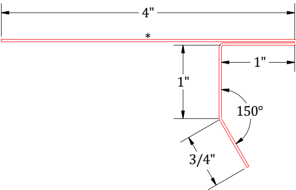
(602A) Flat Eave Trim
