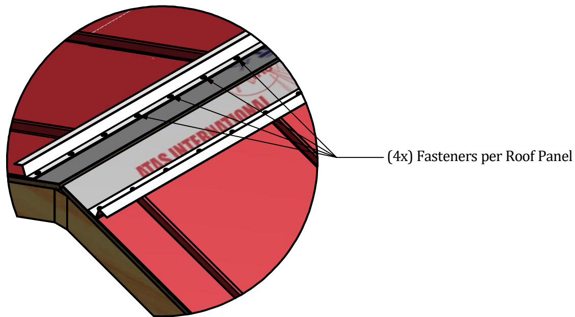
DETAIL - A
