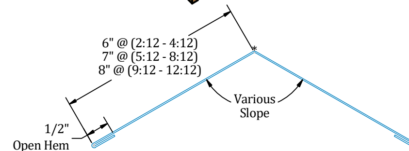
(630.1U/V/W) Ridge Cap
