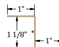
(140PB) Z-Closure
