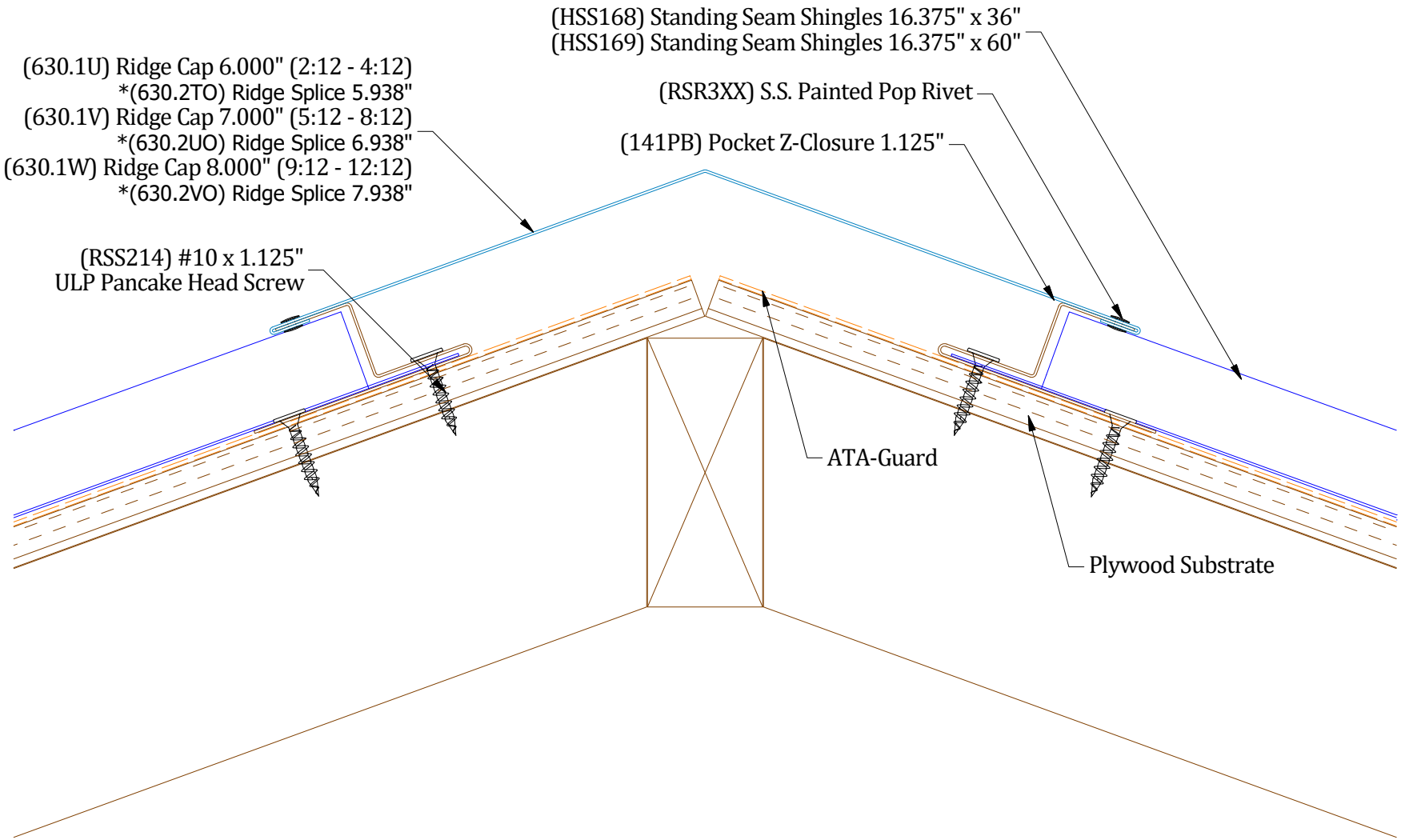
DETAIL - A
