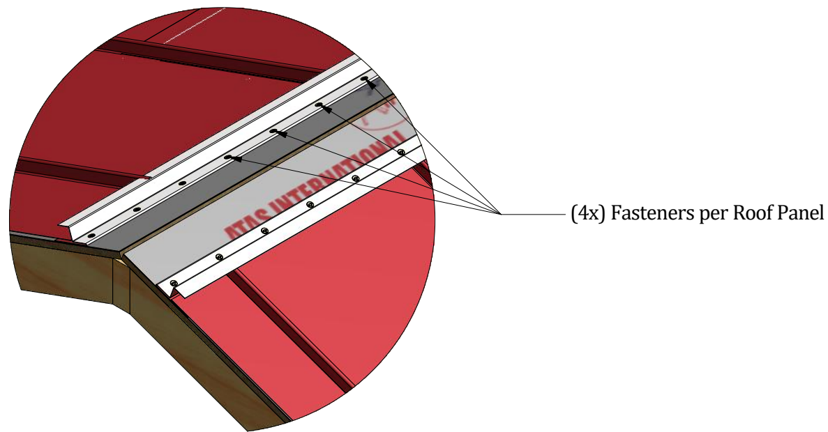
DETAIL - A
