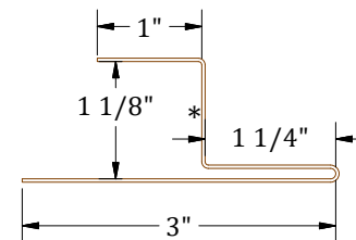
(141PB) Pocket Z-Closure
