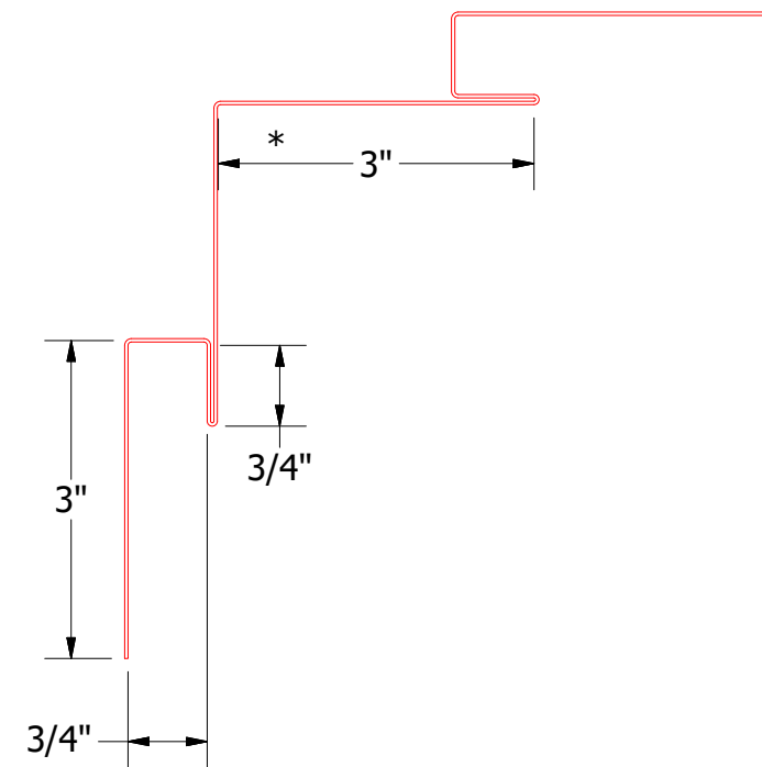
MFA601 - Inside Corner Post
