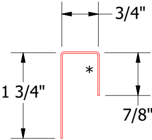
MFA270 - J Closure
