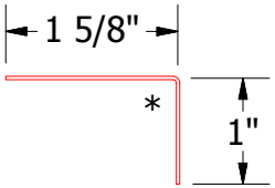
MCA680 - Angle Trim
