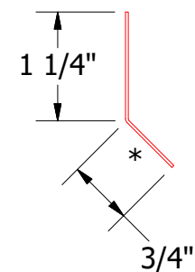
MCA995 - Starter Cleat
