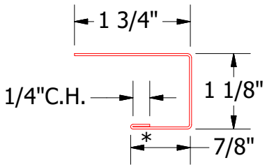
MCA118 - J Channel
