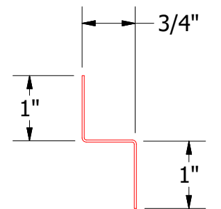
MCA681 - Support Z
