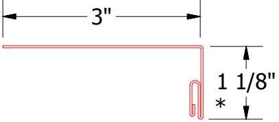
MCA119 - Snap J Base
