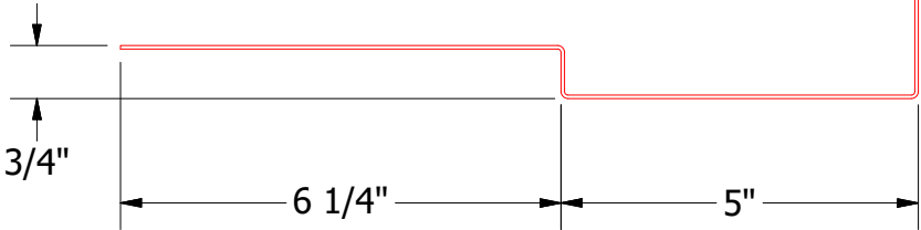
Support Plate
