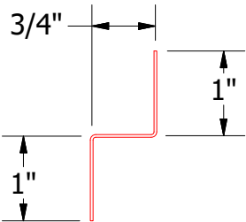
MCA681-Support Z
