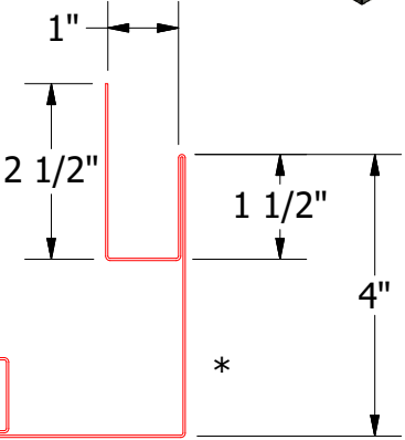
MCA602-Outside Corner Post
