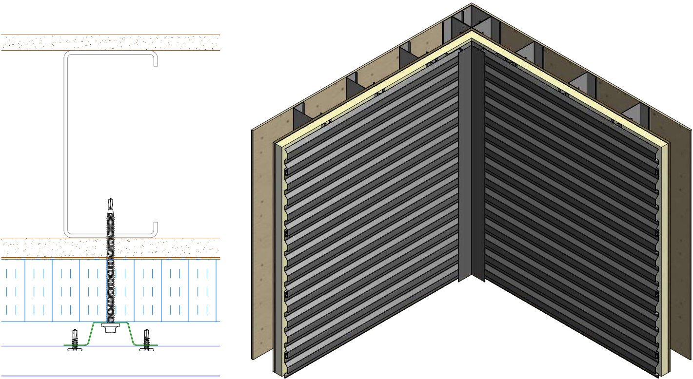
Alternate Subgirt Orientation
