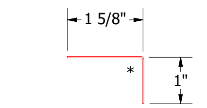
MCA680-Angle Trim
