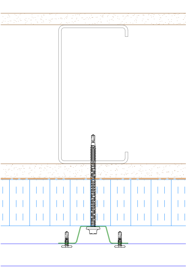
Alternate Subgirt Orientation (NTS)
