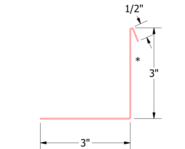
MCA683-Angle with Return
