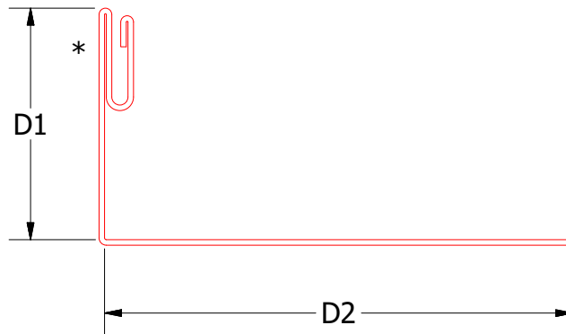
Snap Base
