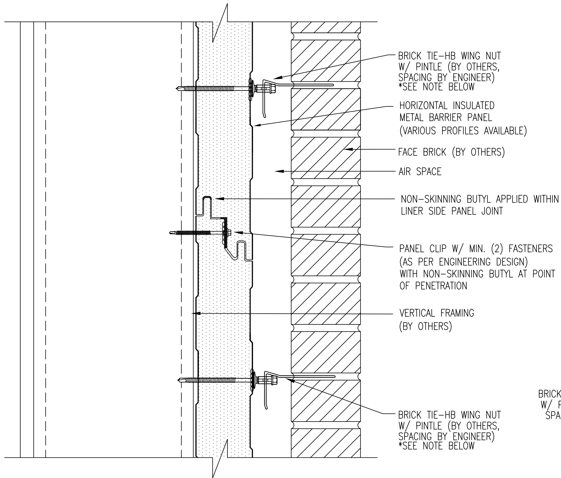
-Section View-
