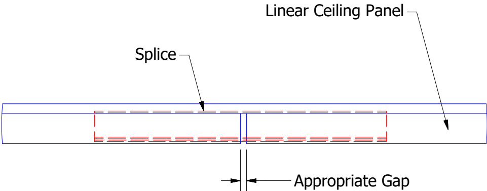
DETAIL A
