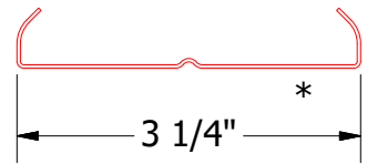
Splice for LCB338
