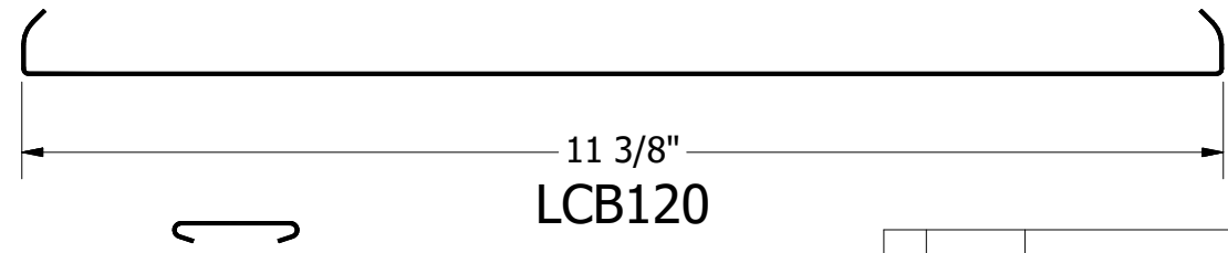
Recessed Filler Strip
