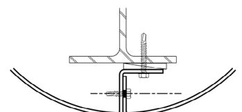
VERTICAL CURVED JOINT
