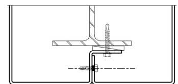
VERTICAL FORMED JOINT
