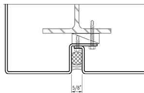
VERTICAL CURVED JOINT WITH REVEAL
