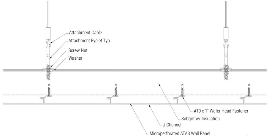
Suspended Horizontal Panel
