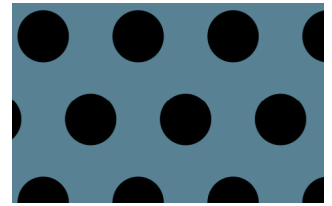
A23 \frac{1}{4} " holes | \frac{1}{2} " staggered centers 23% open area
