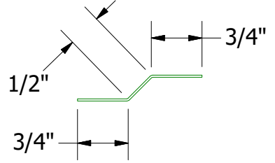
Joggle Cleat DWA975 DSA975
