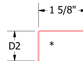
Angle Trim DWA680: D2 = 1" DSA680: D2 = 1 1/2"
