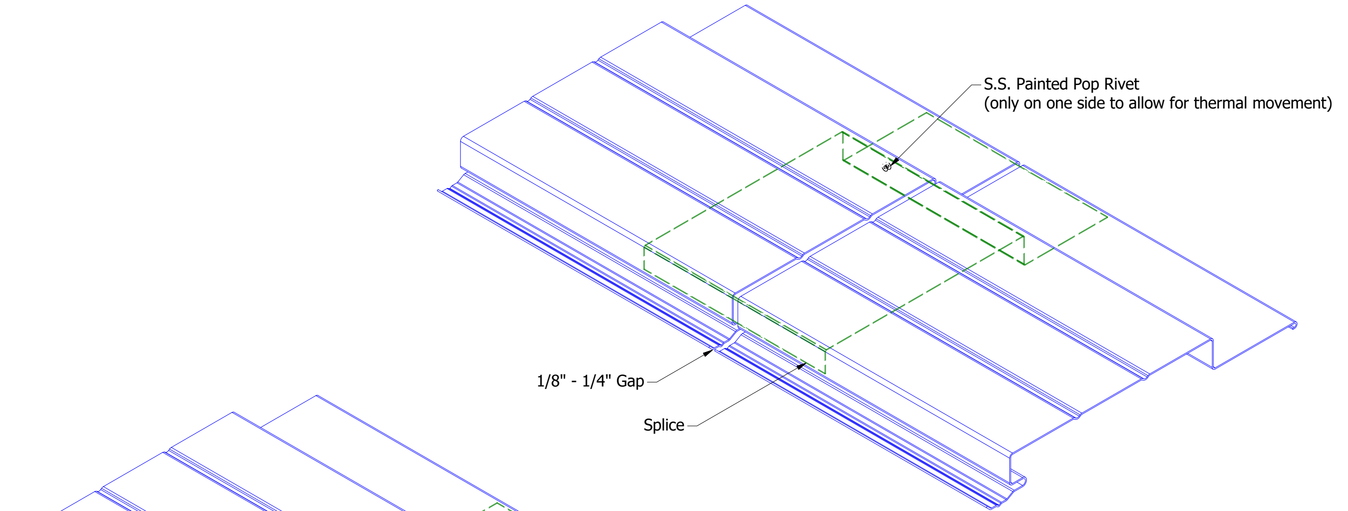
Pop Rivet Splice Detail
