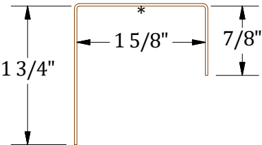
J-Closure
