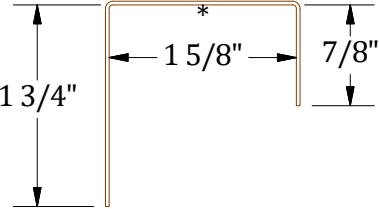
J-Closure
