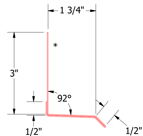
Base Trim
