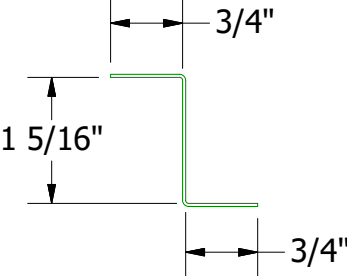
Support Z
