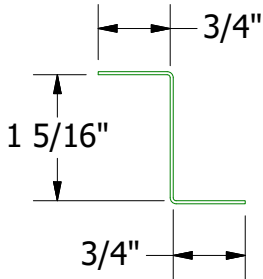
Support Z
