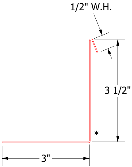
Angle Trim with Return
