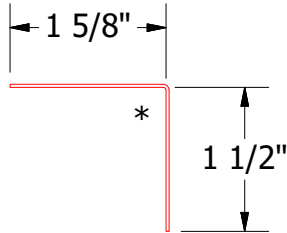
Angle Trim
