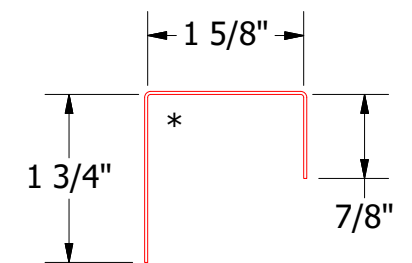
J Closure
