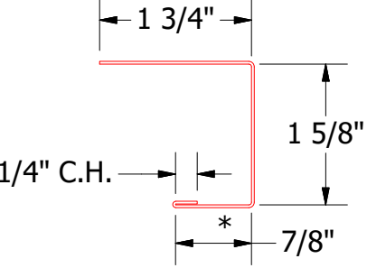
J Channel
