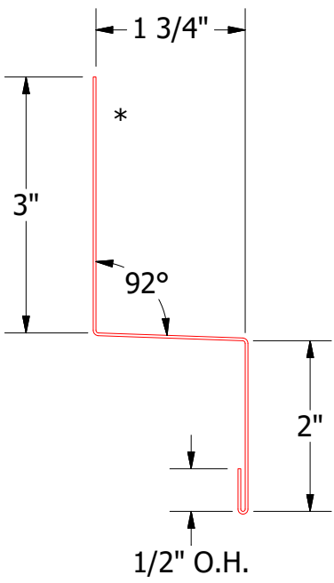
Head Trim
