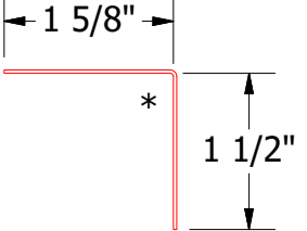
Angle Trim
