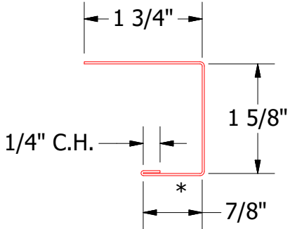
J Channel
