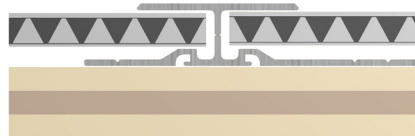
1-Piece, Tight-Fit Flush H Extrusion
