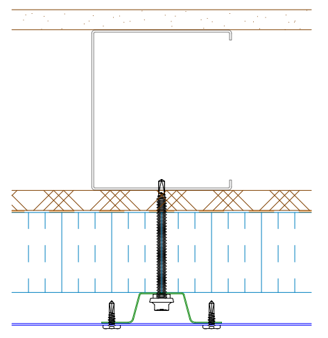
Alternative Subgirt Orientation
