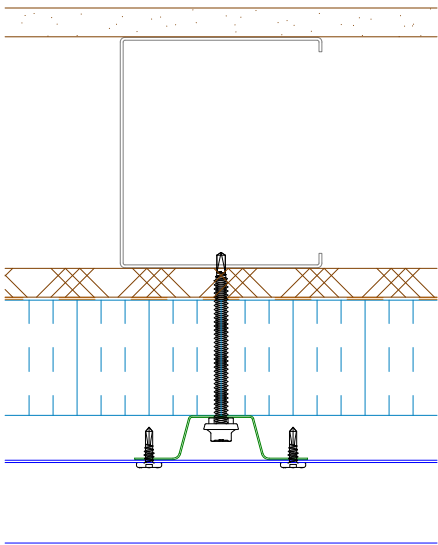
Alternative Subgirt Orientation
