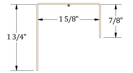
J-Closure
