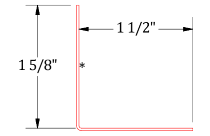
Angle Trim
