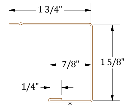
J-Channel
