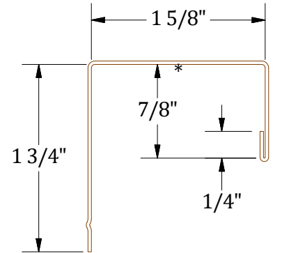
J-Channel
