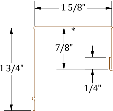
J-Channel
