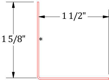
Angle Trim
