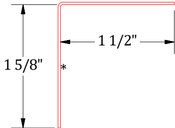
Angle Trim
