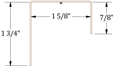
J-Closure
