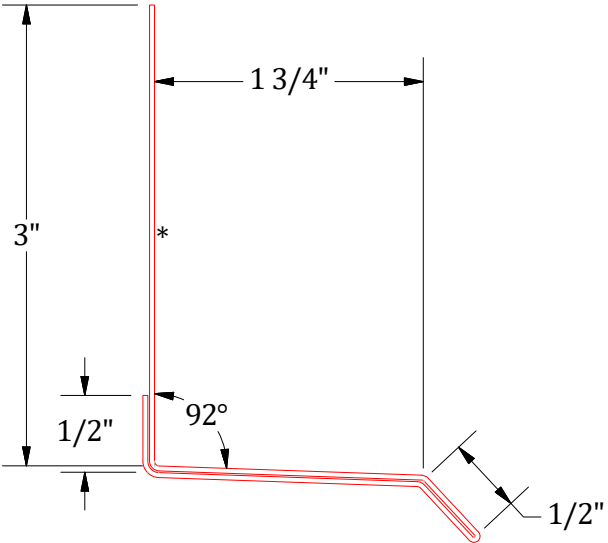
Base Trim w/ Return
