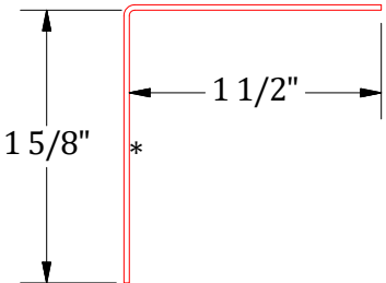
Angle Trim
