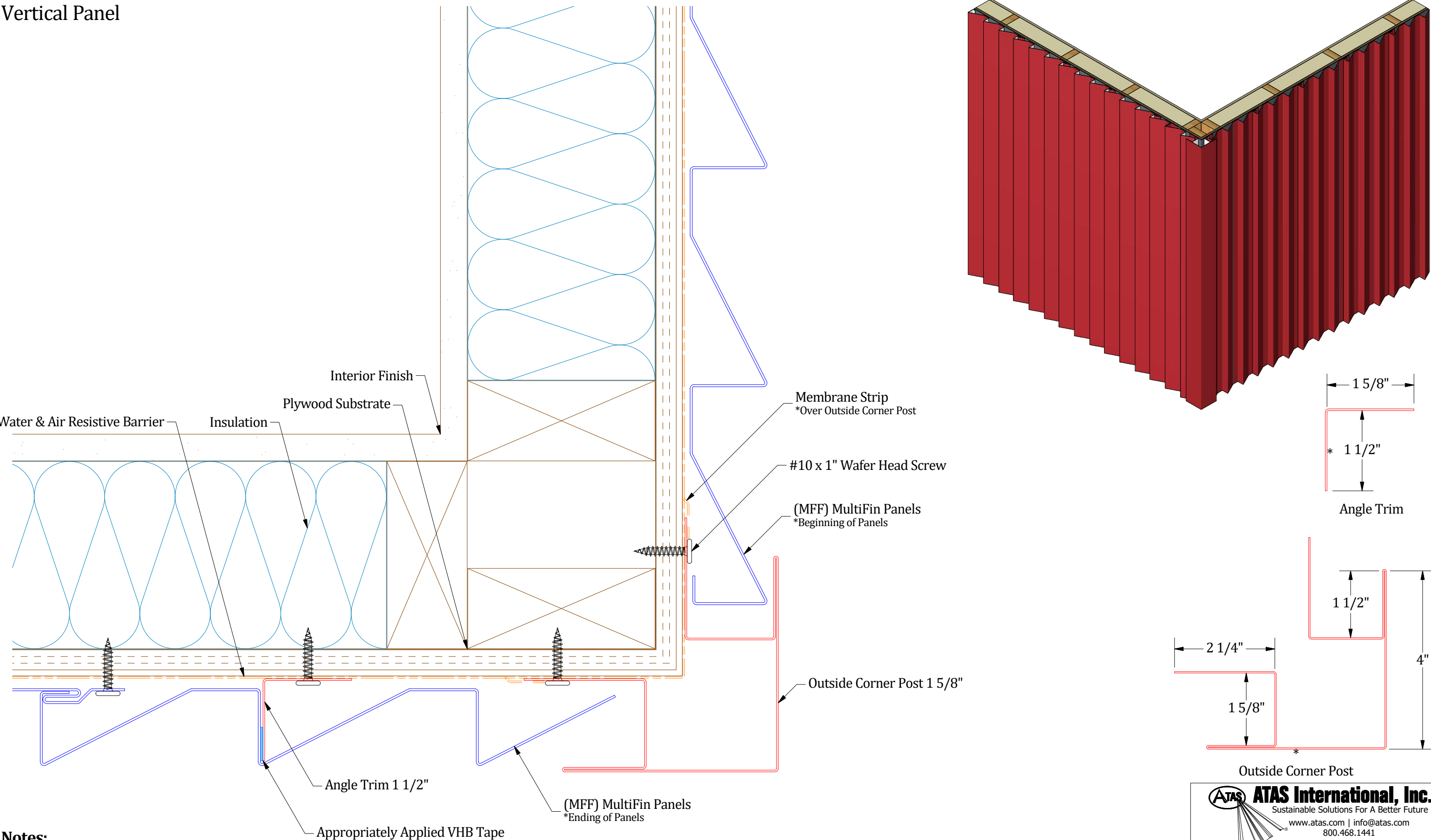
Outside Corner Post Detail
