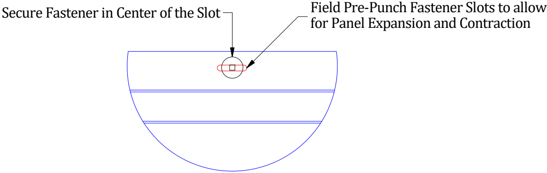
DETAIL A
