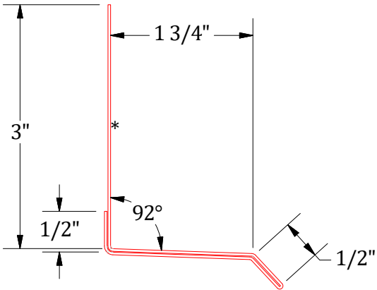
Base Trim w/ Return
