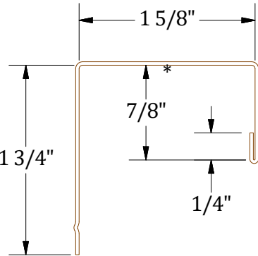
J-Channel
