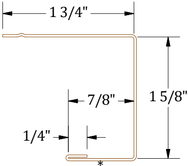
J-Channel
