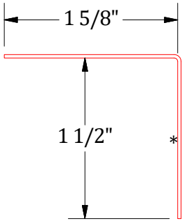
Angle Trim
