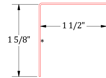
Angle Trim
