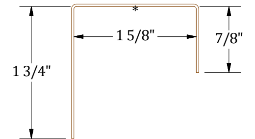
J-Closure
